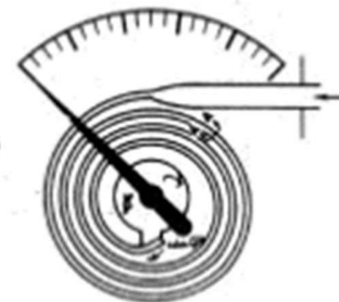
Coiled Bourdon
