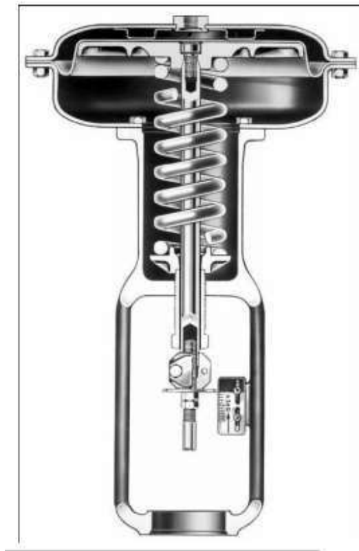
DIRECT-ACTING
