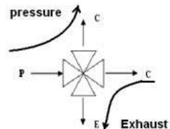
Energised
