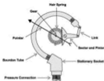
"C" Type Bourdon
