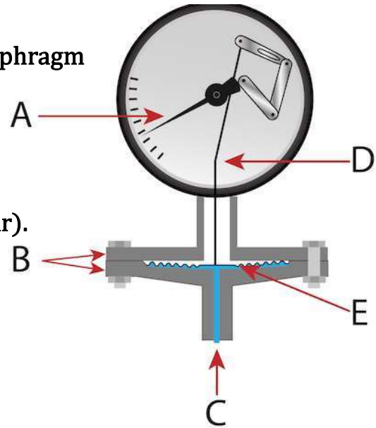
Figure 2: Operating principle of a diaphragm pressure gauge: pointer (A), upper and lower housing (B), pressure inlet (C), pressure element (D), and diaphragm (E).
