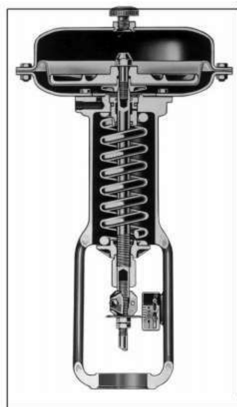
REVERSE-ACTING
