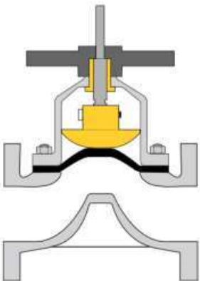
Diaphragm Valve
