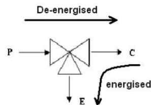
Normally open
