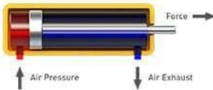
Double Acting Cylinder Position 1
