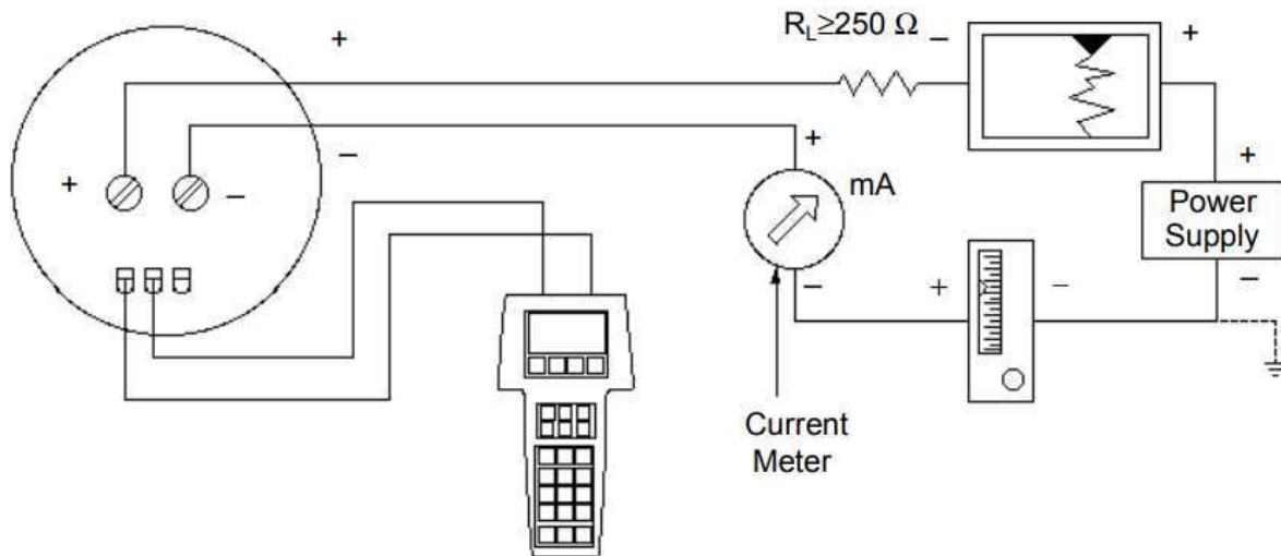
FIGURE 1-3. Connecting to the Transmitter Comm Terminals.
